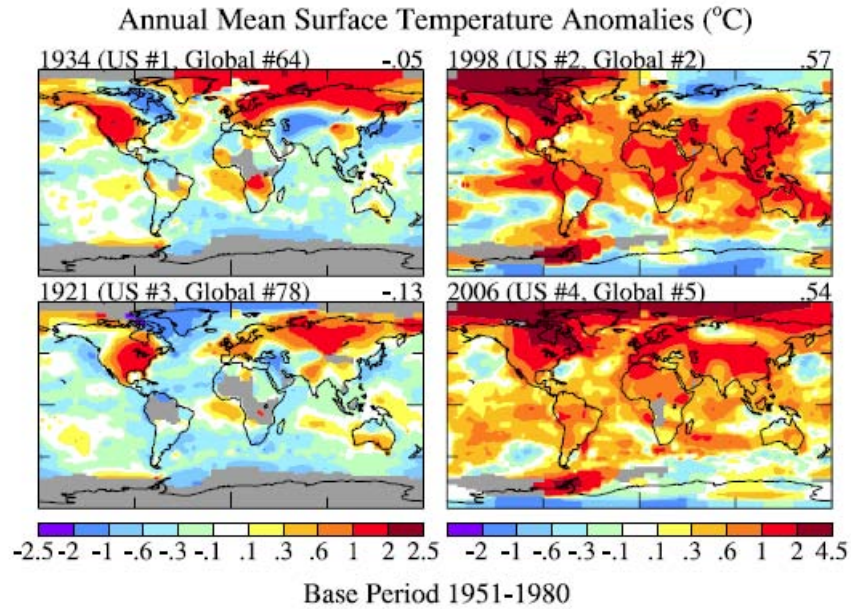
Figure 2. Temperature anomalies, relative to 1951-1980 base period, in the four years that are the warmest in the contiguous U.S. in the GISS analysis.
