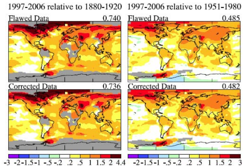
Figure 3. Surface temperature anomalies in the past 10 years (1997-2006) relative to two alternative base periods, 1880-1920 on the left and 1951-1980 on the right. The top row versus the bottom row shows the effect of the data flaw.
