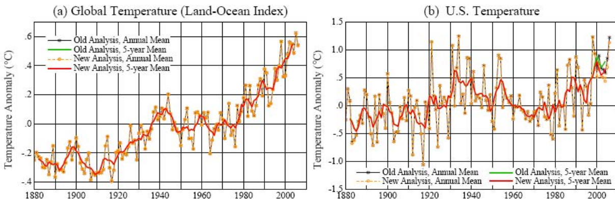
Figure 1. Global (a) and U.S. (b) before and after correction of flaw in computer program.
